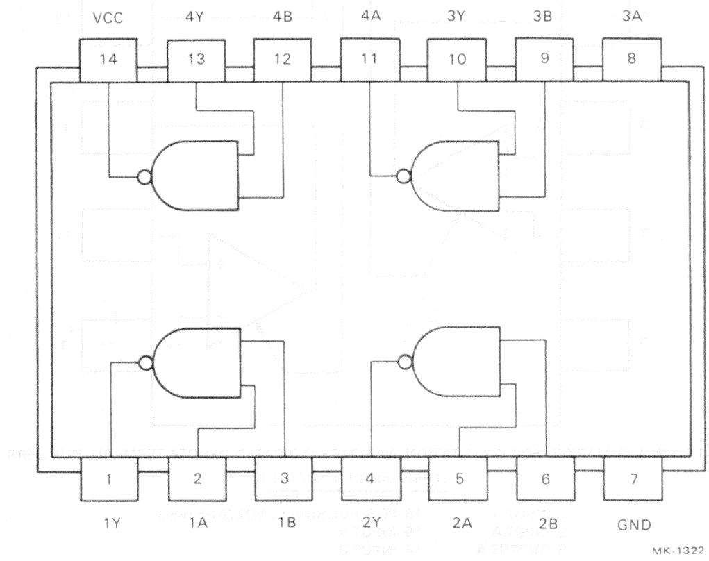
Figure C-6 8881 Pin Identification
