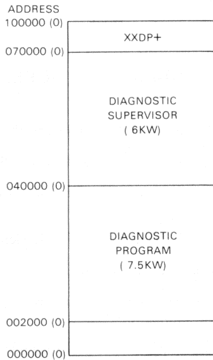
Figure A-1 Typical XXDP+/Diagnostic Supervisor Memory Layout
