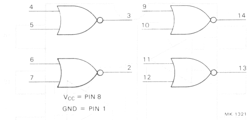
Figure C-5 8640 Equivalent Logic Diagram
