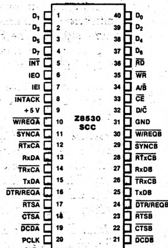
Figure 2. Pin Assignments
