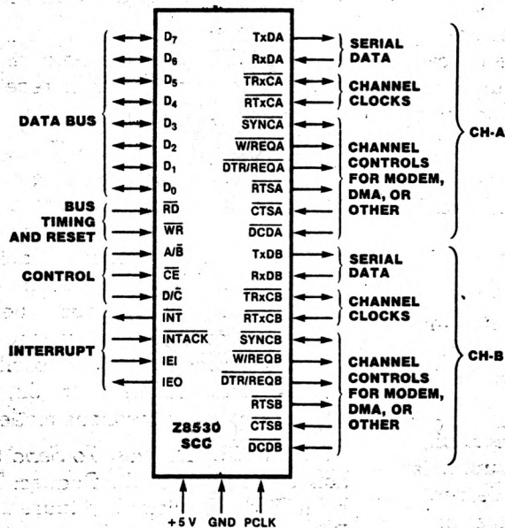
Figure 1. Pin Functions
