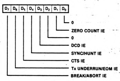
Figure 10. Read Register Bit Functions
